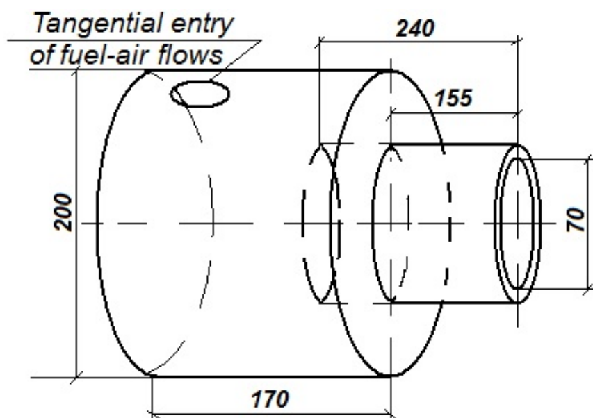
FIGURE 1 – Burning device drawing
