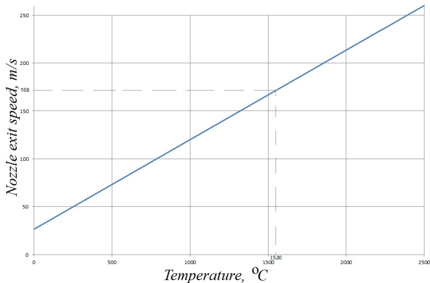
FIGURE 4 – The dependence of the speed of the output gases from the combustion temperature
